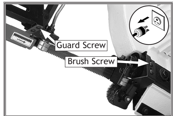
Figure 38. Blade accessories.
